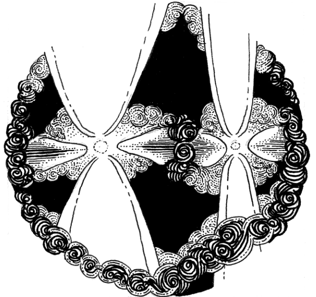
Non-Coeval
