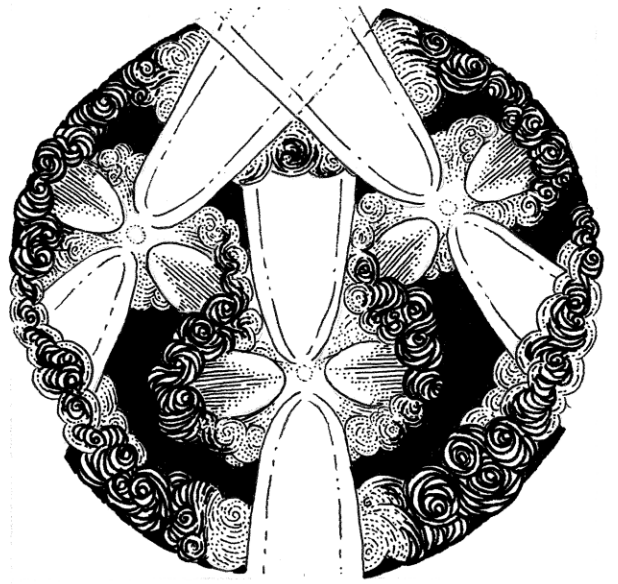
Multiple Protostellar System
