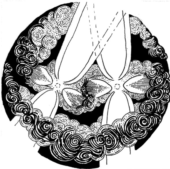
Coeval
