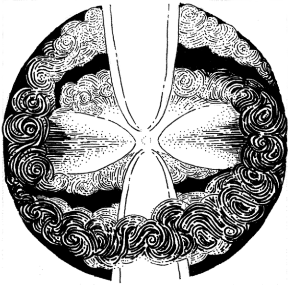
Single Protostellar System
