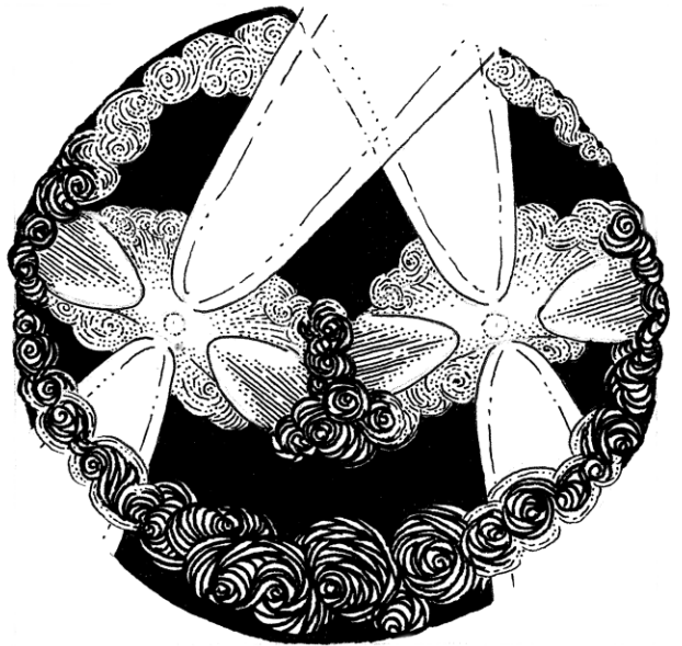
Position Angle
