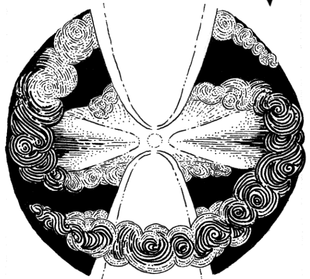
Class I
