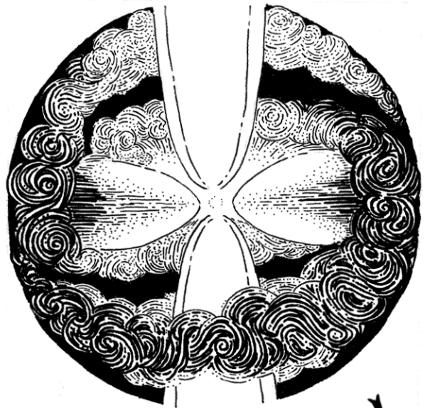
Class 0
