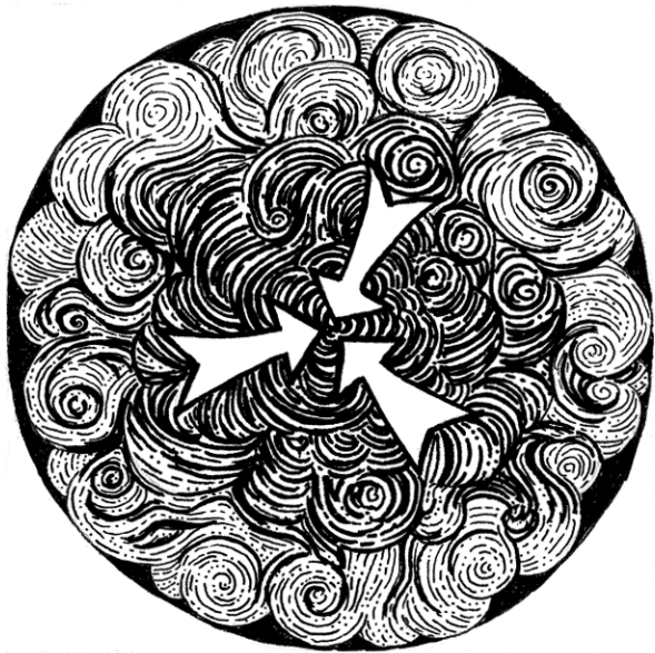
Starless Core
