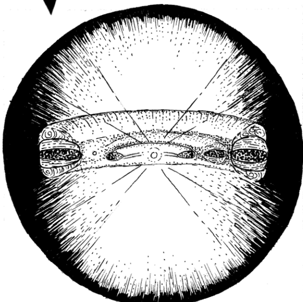
Class III
