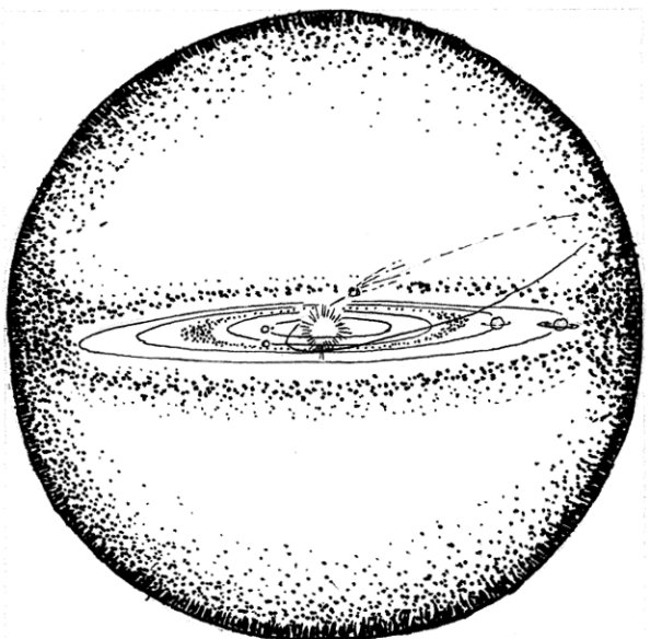
Star-Planet System
