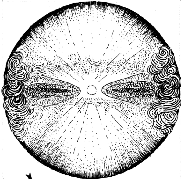
Class II
